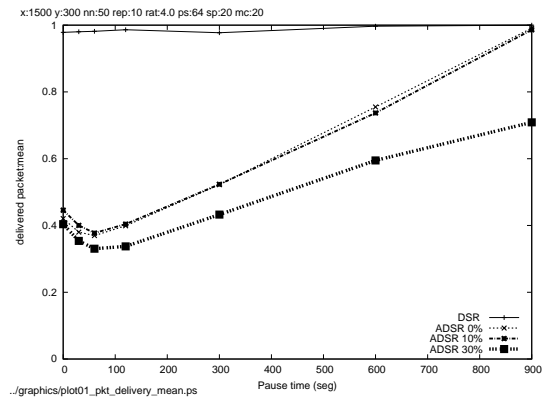
Fig. 6. Packet Delivery
