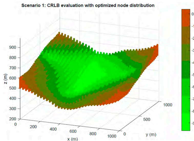
Figure 6. Optimization in Scenario 1. CRLB in meters for TLE region based on node location optimized by GA.
