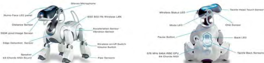
Fig. 1. Sony AIBO ERS7. (image from AIBO site)
