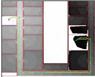
Figure 2: Gradient propagation
