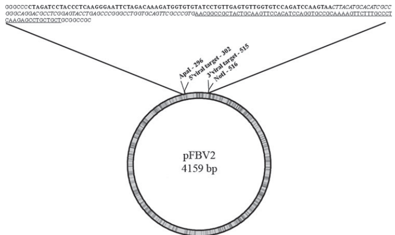
Fig. 2 Graphic representation of pFBV2 containing the sequence of the synthetic DNA. The length of the plasmid is 4,159 bp. The viral insert was flanked by Apa I and Not I sites. The sequences of the qPCR assays are shown (BPvV— bold , HAdV— italics and PAdV— underlined ). The sequences corresponding to the TOPO vector are in normal type
