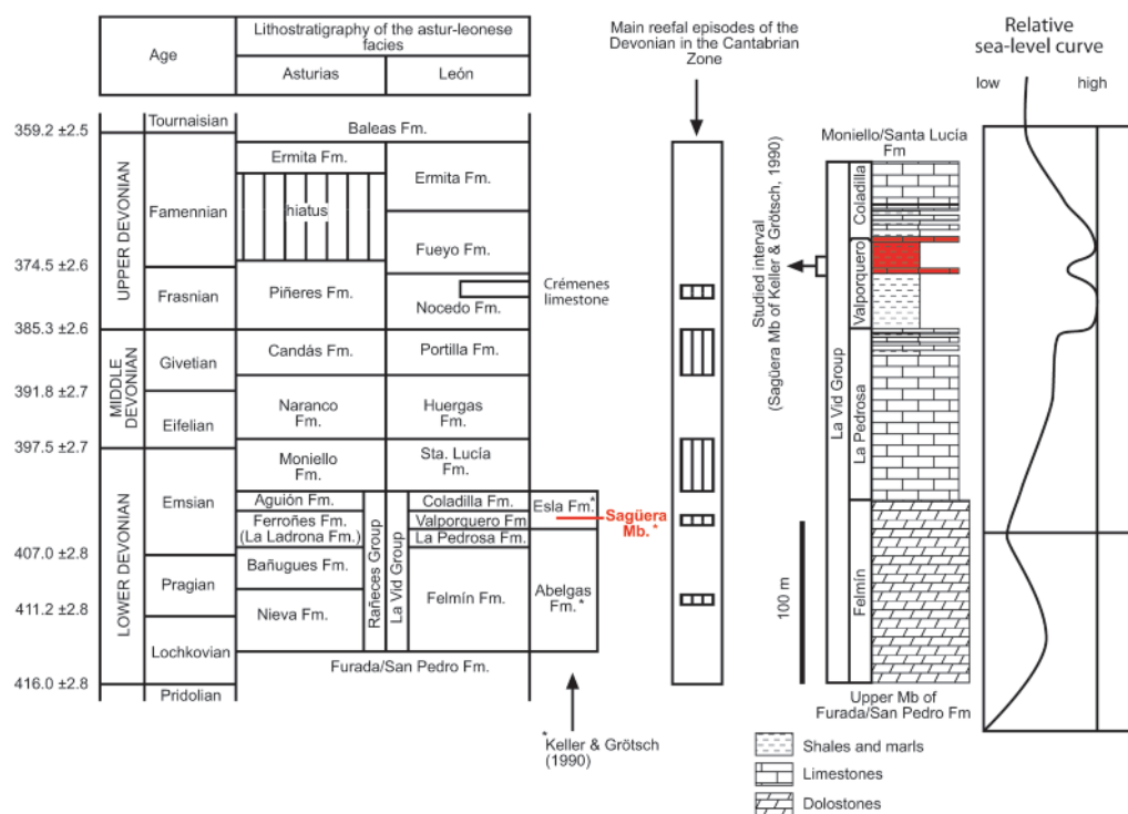
Figure 37. Chronostratigraphic chart showing the Devonian lithostratigraphic units of the Asturo-Leonese facies that have been defined in the political regions of Asturias (northern part of the Cantabrian Zone) and León (southern part of the Cantabrian Zone) and the distribution of the reefal episodes. Absolute ages based on Gradstein et al. (2004). The stratigraphic subdivision of the La Vid Group is that of Vilas Minondo (1971) and Vera de la Puente (1989), but subdivisions by Leweke (1982) and Keller (1988) are also shown. Note that, contrary to other authors, Leweke (1982) treats La Vid Group as a formation made up of members. The log on the right depicts the interpreted relationships between the general stratigraphy of the La Vid Group and the sea-level curve (based on Keller and Grötsch 1990) and shows the location of the studied interval of the Valporquero Formation. After Fernández et al. 2006.
