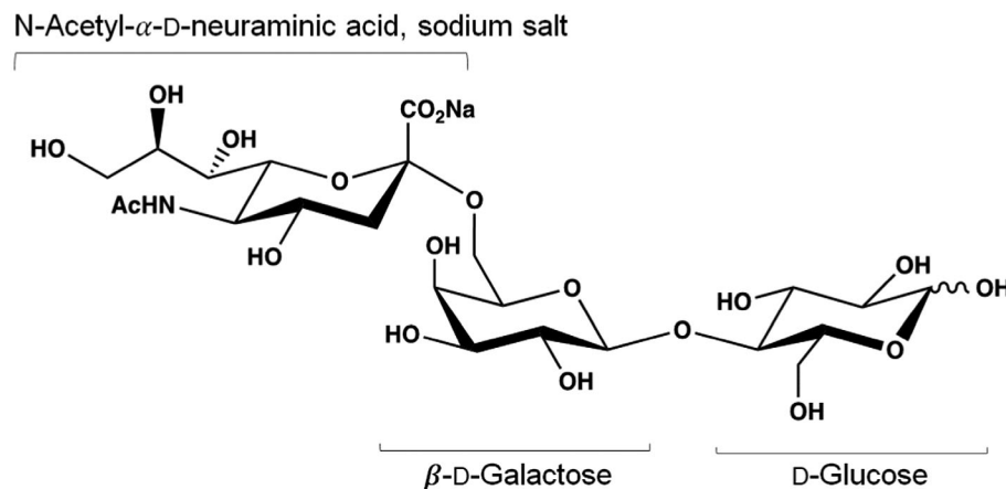
Figure 1: Chemical structure of 6'-SL sodium salt (EFSA NDA Panel, 2022a)
