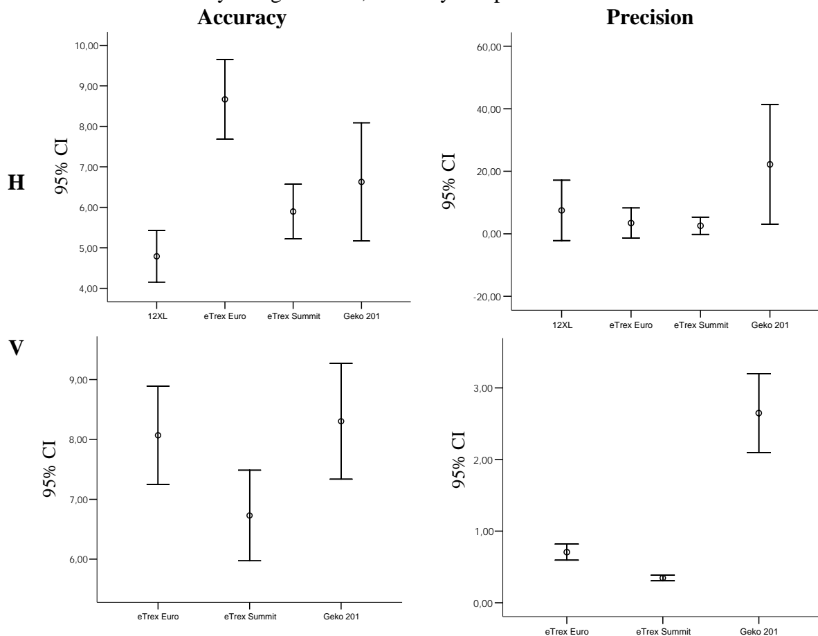
Figure 2. Error bars with the confidence intervals at 95% for horizontal (H) and vertical (V)
