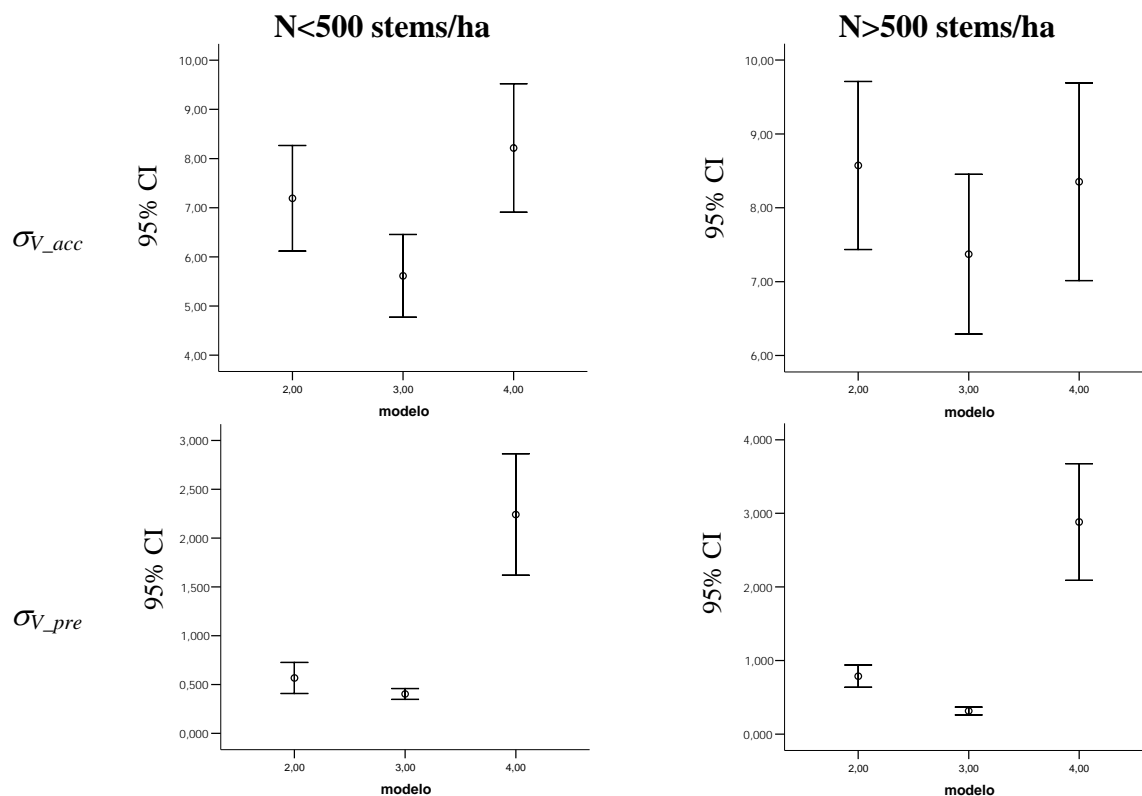
Figure 4. Error bars with the confidence intervals at 95% for horizontal accuracy and precision, regarding receivers and stand density.
