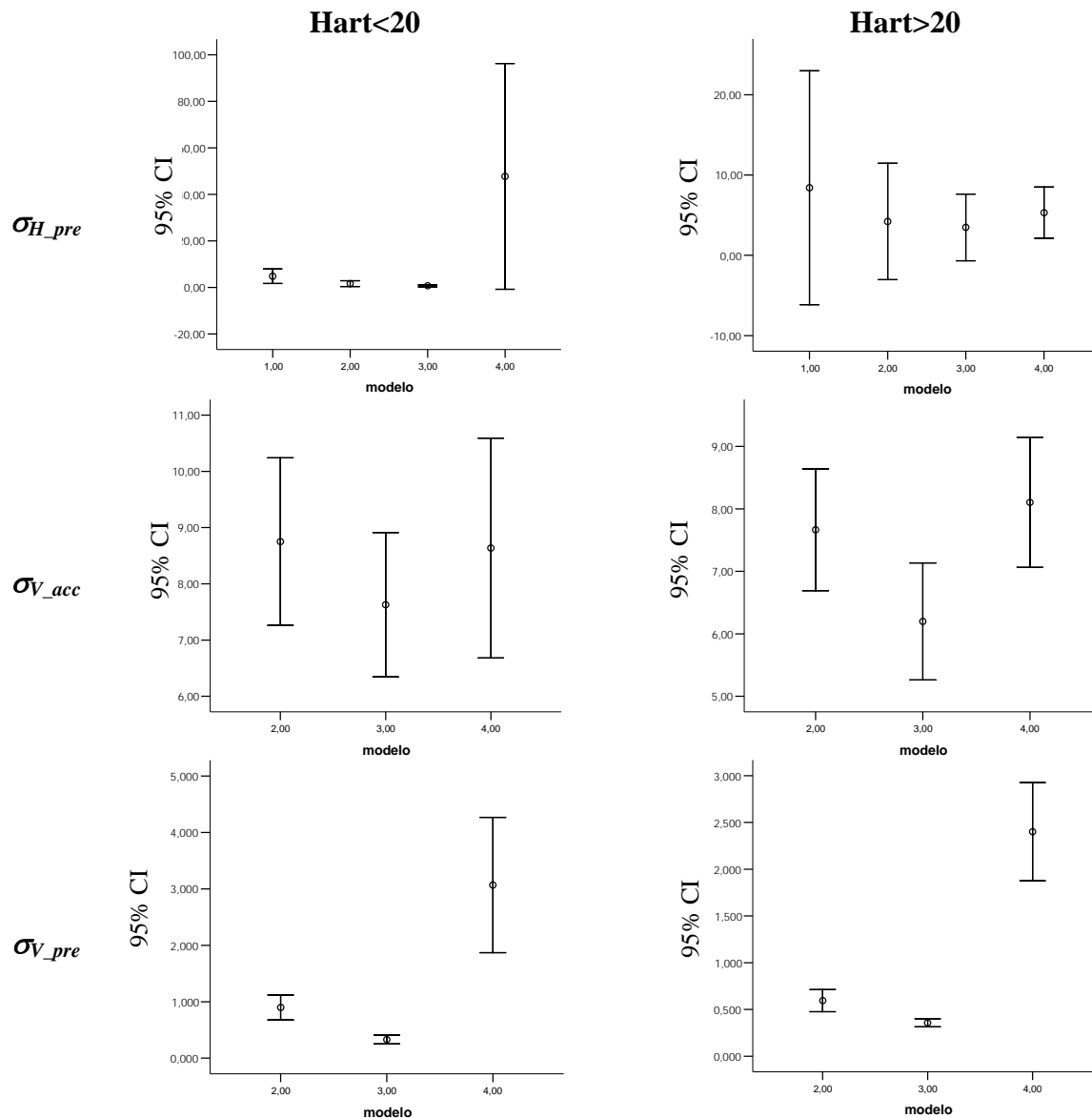
Figure 5. Error bars with the confidence intervals at 95% for horizontal accuracy and precision, regarding receivers and Hart-Becking index.
