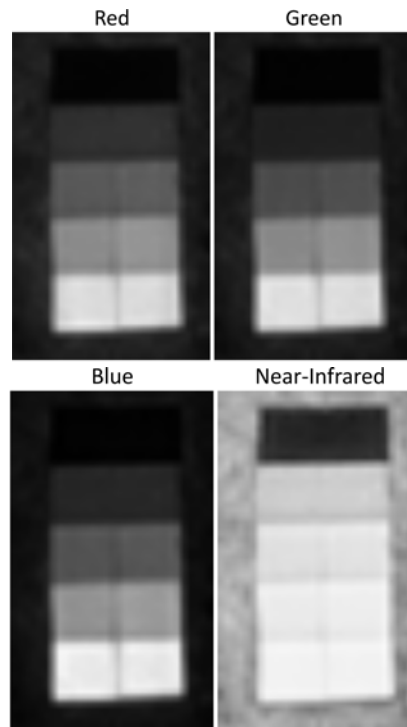
Figure 1. Portable reflectance targets (0%, 25%, 50%, 75% and 100% nominal reflectance) placed in the field (orthophoto 7017)
